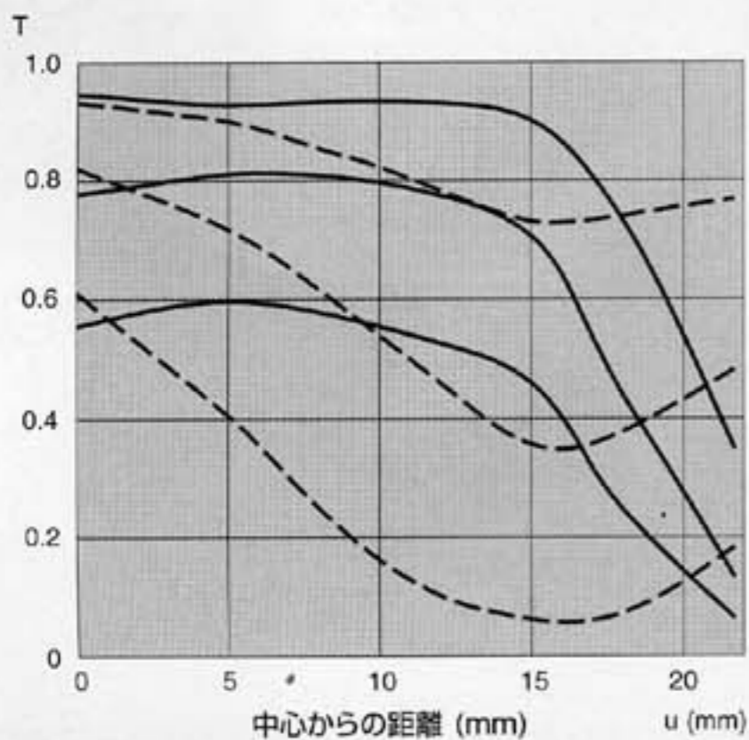
図1 MTF (F3.5)
